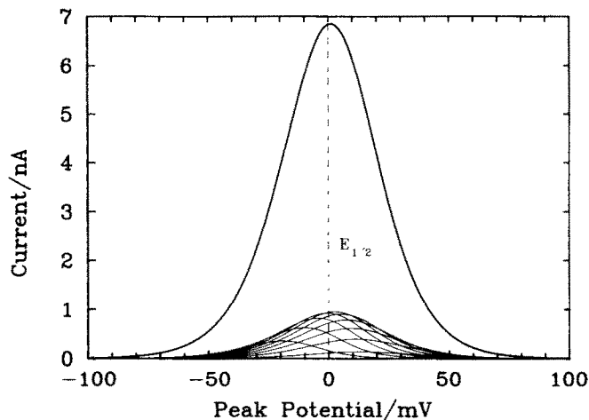
Fig. 6. Approximation of the stripping peak for a 40 \mu\text{m} thick semi-spherical mercury film, by combining the stripping peaks of ten annular flat films (conditions given in text).
