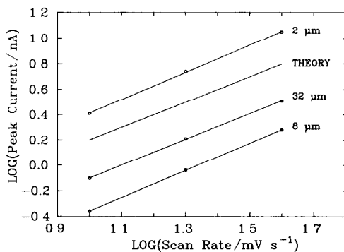
Fig. 1. Log-log dependence of the peak current ( i_p ) on the scan rate ( v ), for different film thicknesses. Theoretical curve is for \alpha = 1 .
