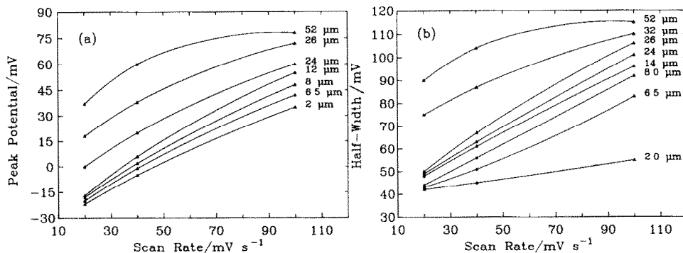
Fig. 2. Effect of scan rate on ASV; (a) peak potential, and (b) peak half-width, for the film thicknesses indicated.
