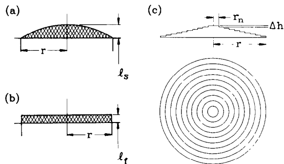
Fig. 5. Relationship between; (a) an equivolume semi-spherical film; and (b) a flat film. (c) Approximation of the semi-spherical film by annular flat films. (Not to scale.)
