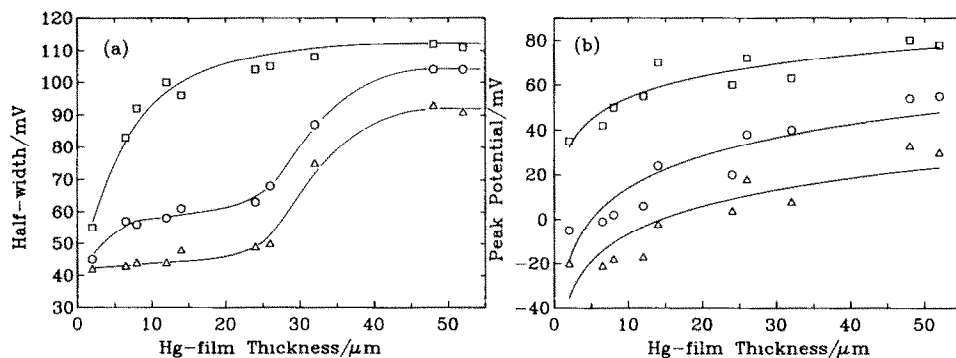
Fig. 3. Effect of mercury film thickness on ASV; (a) peak half-width and (b) peak potential. v(\Delta) 20; (○) 40; (□) 100 mV/s; solid curves are best spline fit.
