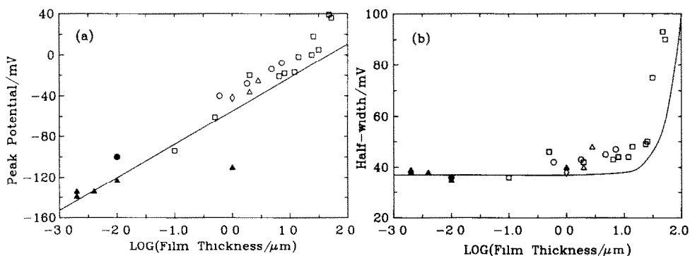
Fig. 4. Comparison of data from both the literature and this work with the theoretical predictions [2,3] for the effect of mercury film thickness on: (a) peak potential, and (b) peak half-width. v = 20 \text{ mV/s} ; (—) Theory; (●) GC, (▲) graphite, (○) Pt, (△) Ni, (□) Ir, (◇) Ag.
